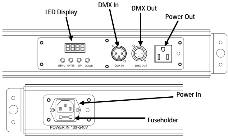
Back Panel View
