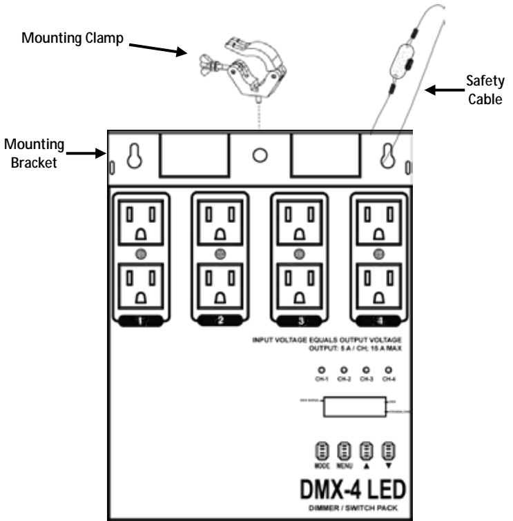
Mounting Diagram
