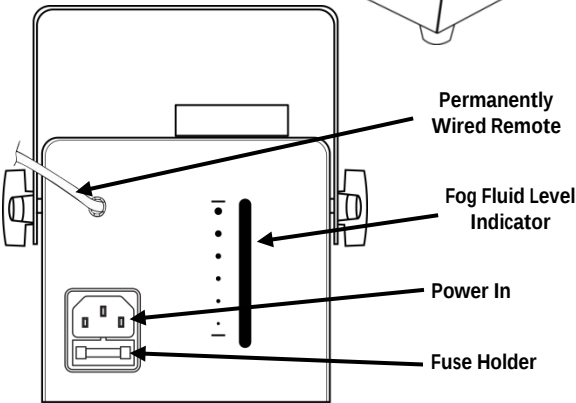
Back Panel View
